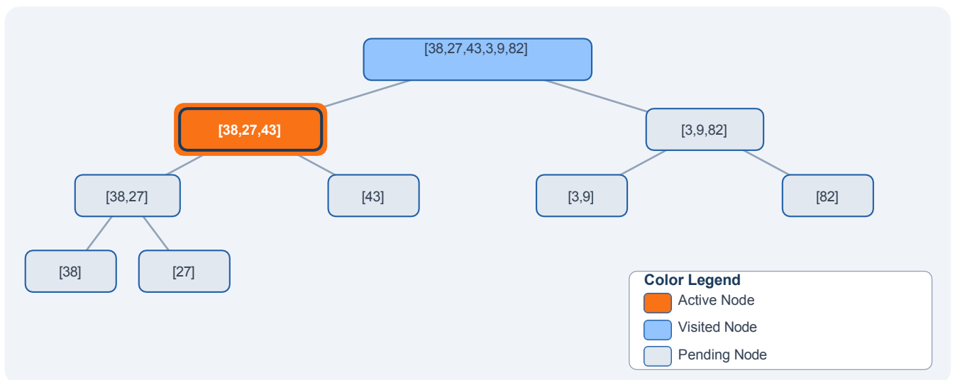
Figure 5: Three-state color-coding scheme. The currently active node is highlighted in orange, visited nodes in light blue, and pending nodes in light gray. Smooth CSS transitions animate state changes.
