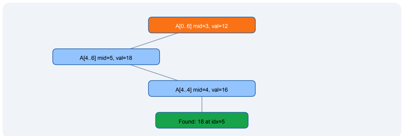
Figure 3: Recursion tree for Binary Search on A=[4,8,12,16,18,21,24] , \text{target}=18 . Tree depth is O(\log n) , illustrating logarithmic search reduction.
