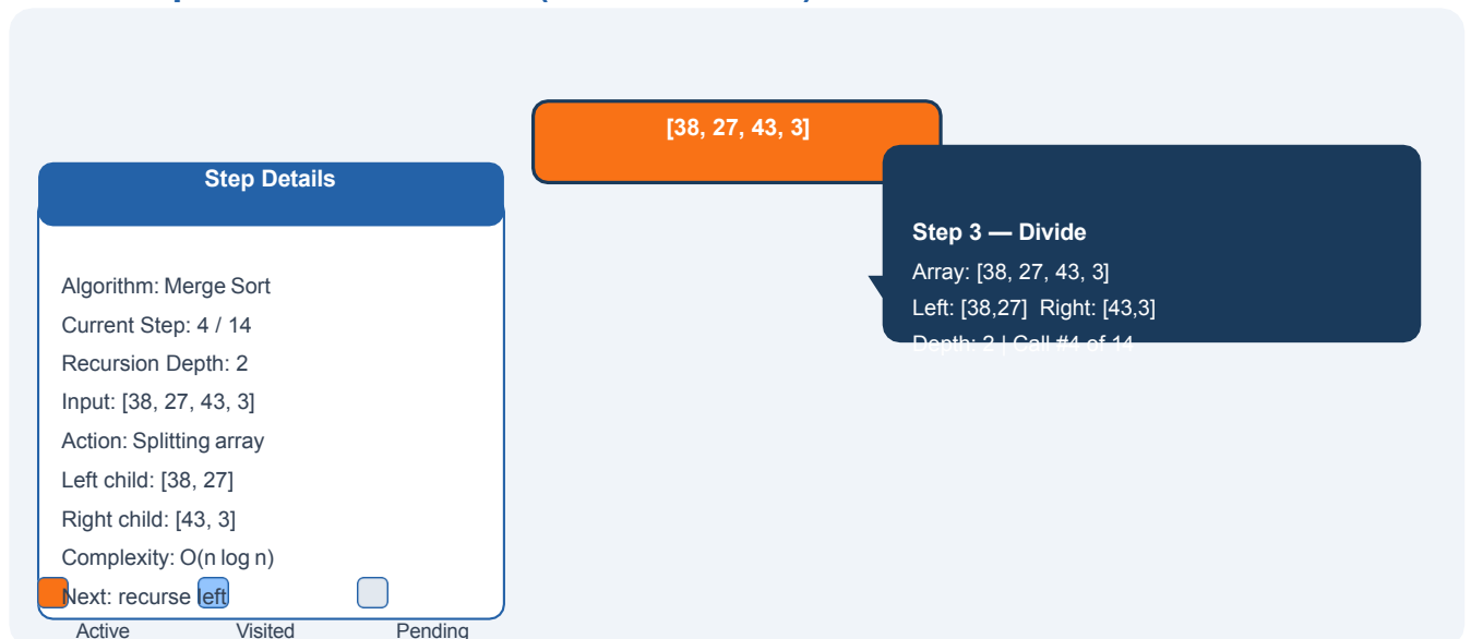
Figure 4: Updated UI showing the side panel (left) with step-by-step annotations and the tooltip bubble (right) appearing on the active node. The color legend is shown at the bottom.
